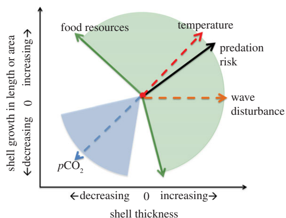
Figure 4. Possible shell length (or area) and thickness responses of a mussel shell to various biotic (solid) and abiotic factors (dashed) represented as vectors. The figure highlights the range of possible shell growth responses to environmental variables, and we suggest that coincident, opposing and interacting [43] environmental variables are possible. The green area designates the range of possible responses to increased food resources, including increases in both length and thickness, while the blue area shows possible negative responses to ocean acidification (e.g. [44]).
